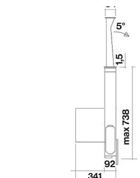
Side view, motor on the back
