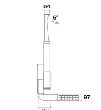
Side view, Slim motor on the back
