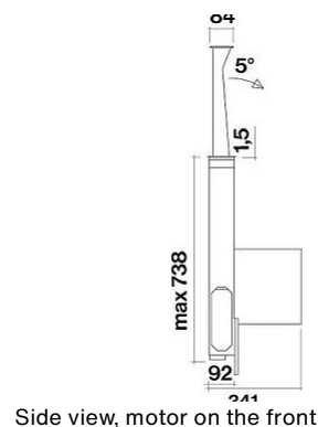
Side view, motor on the front
